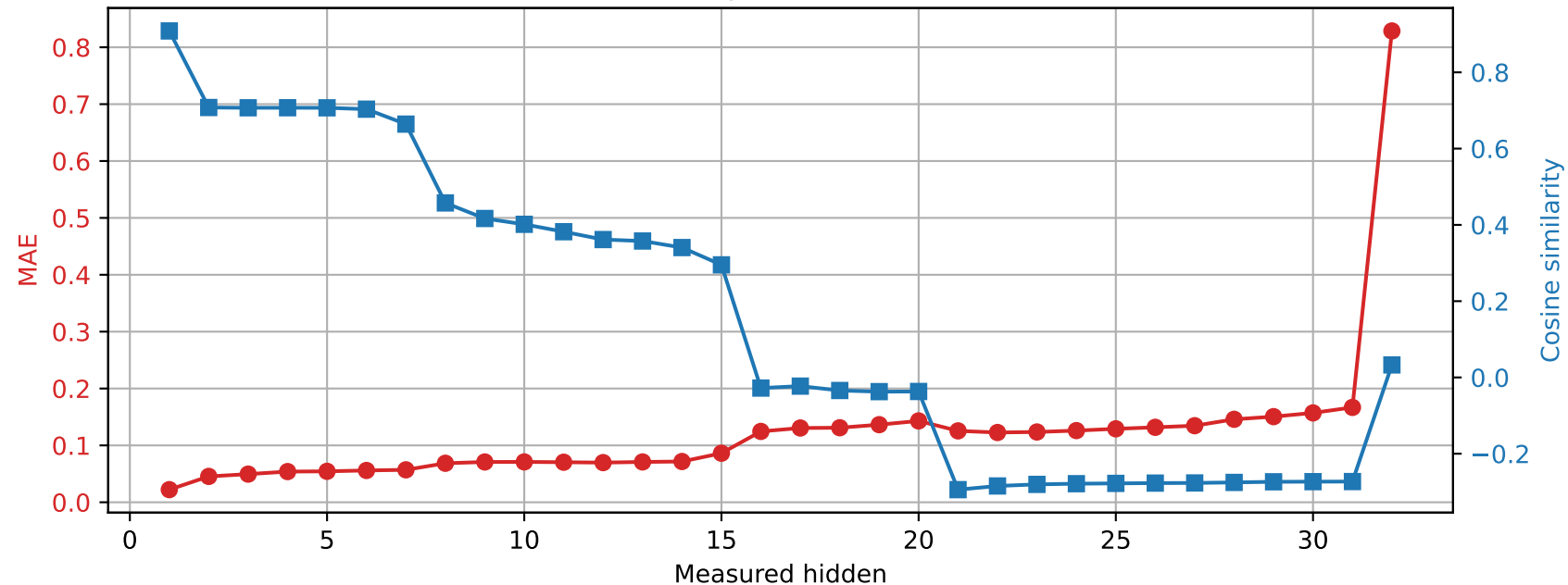
OLMo-7B-hf | Prompt 2 Spared layer 31 | Unquantized vs hybrid
