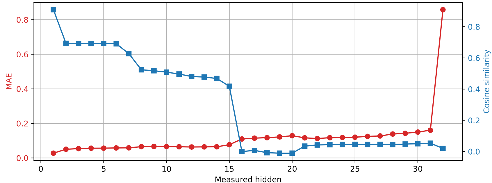
OLMo-7B-hf | Prompt 3 Spared layer 22 | Unquantized vs hybrid
