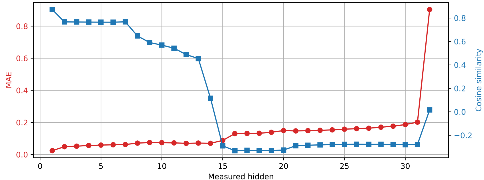
OLMo-7B-hf | Prompt 4 Spared layer 5 | Unquantized vs hybrid
