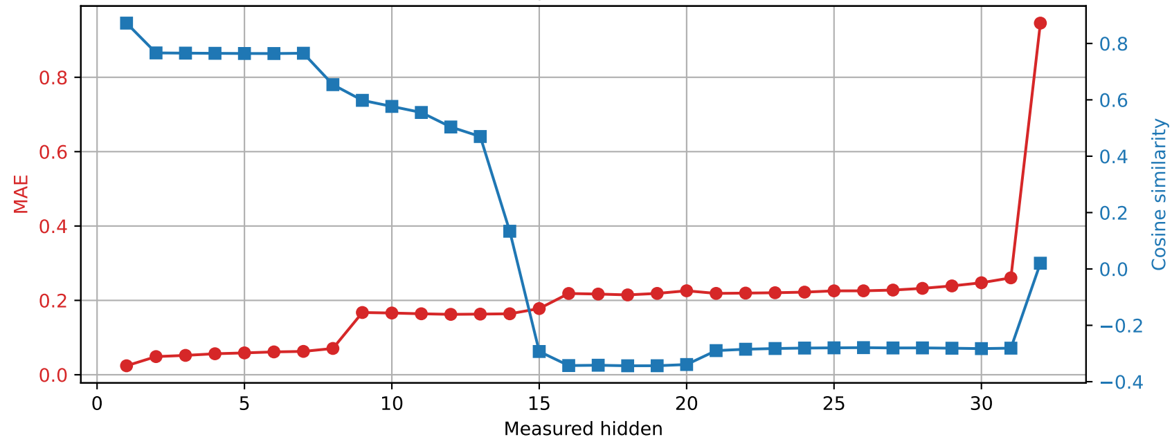
OLMo-7B-hf | Prompt 4 Spared layer 8 | Unquantized vs hybrid
