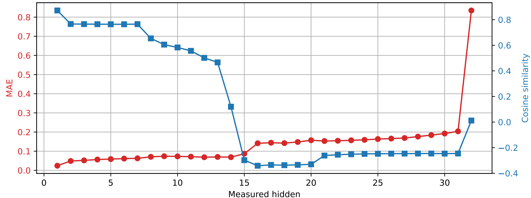
OLMo-7B-hf | Prompt 4 Spared layer 15 | Unquantized vs hybrid
