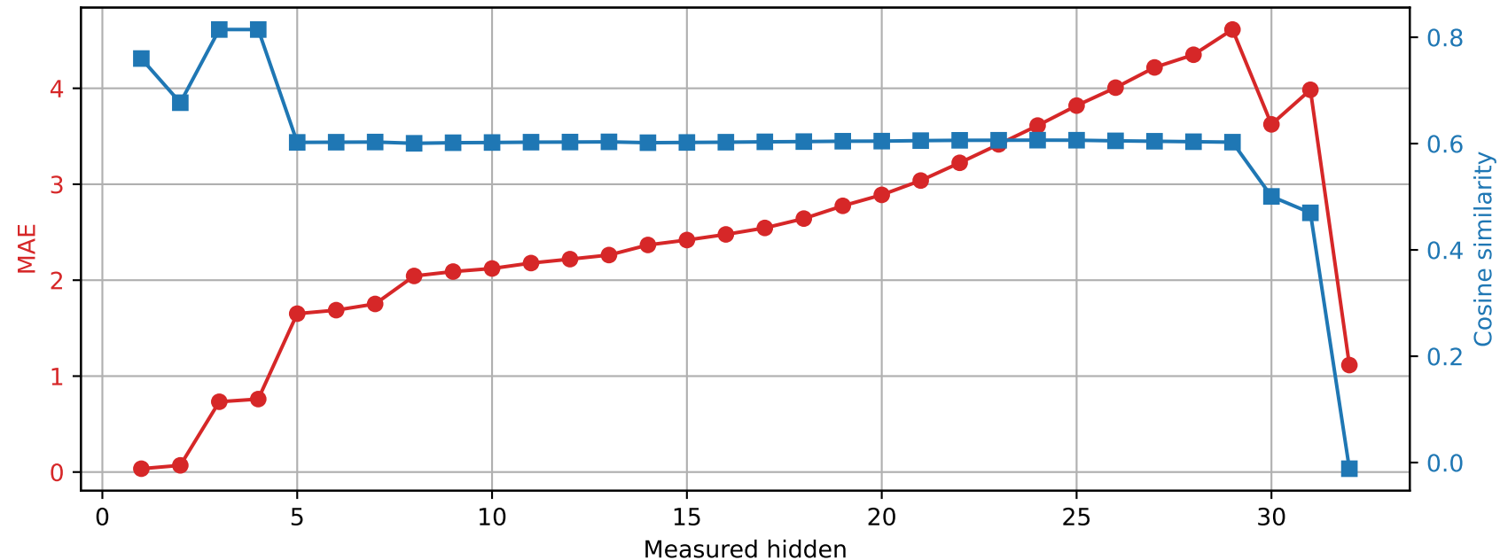
Phi-3-mini-4k-instruct | Prompt 0 Unquantized vs quantized int4
