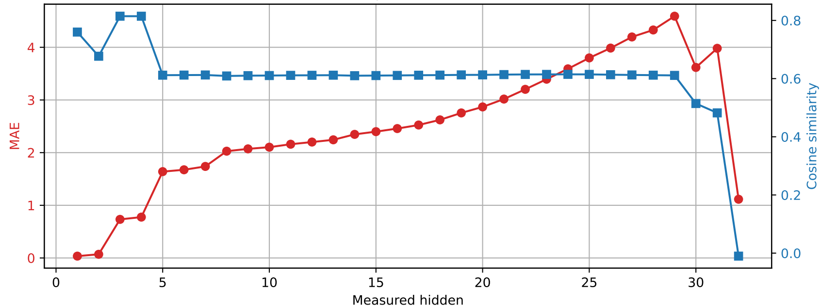
Phi-3-mini-4k-instruct | Prompt 0 Spared layer 3 | Unquantized vs hybrid
