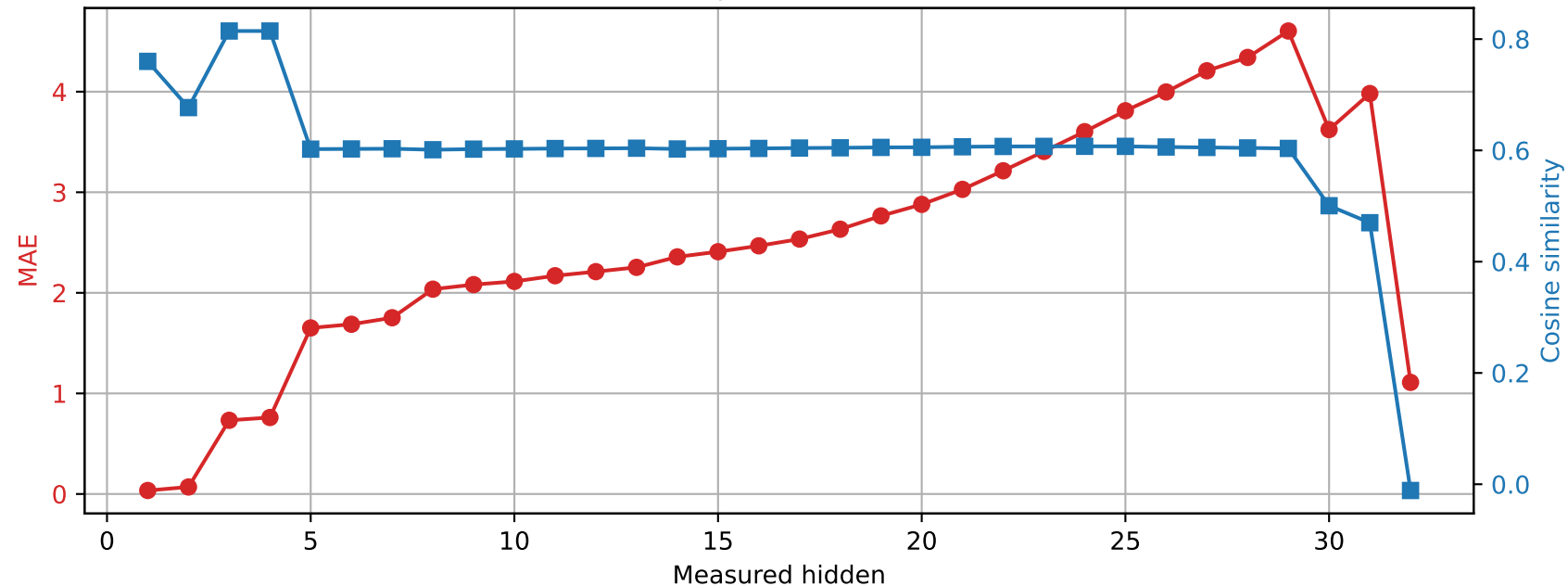
Phi-3-mini-4k-instruct | Prompt 0 Spared layer 5 | Unquantized vs hybrid
