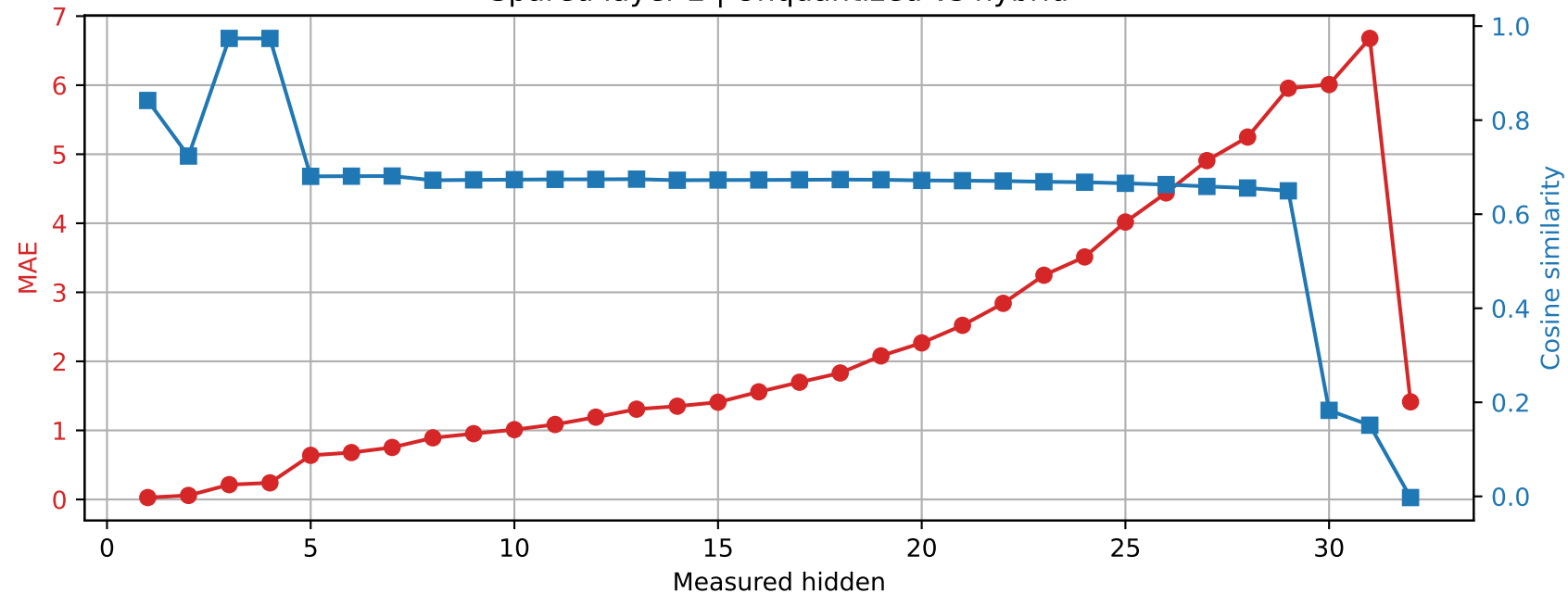
Phi-3-mini-4k-instruct | Prompt 1 Spared layer 2 | Unquantized vs hybrid
