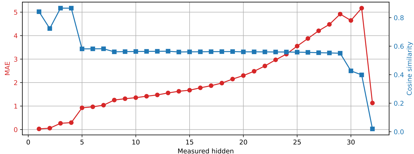
Phi-3-mini-4k-instruct | Prompt 1 Spared layer 5 | Unquantized vs hybrid
