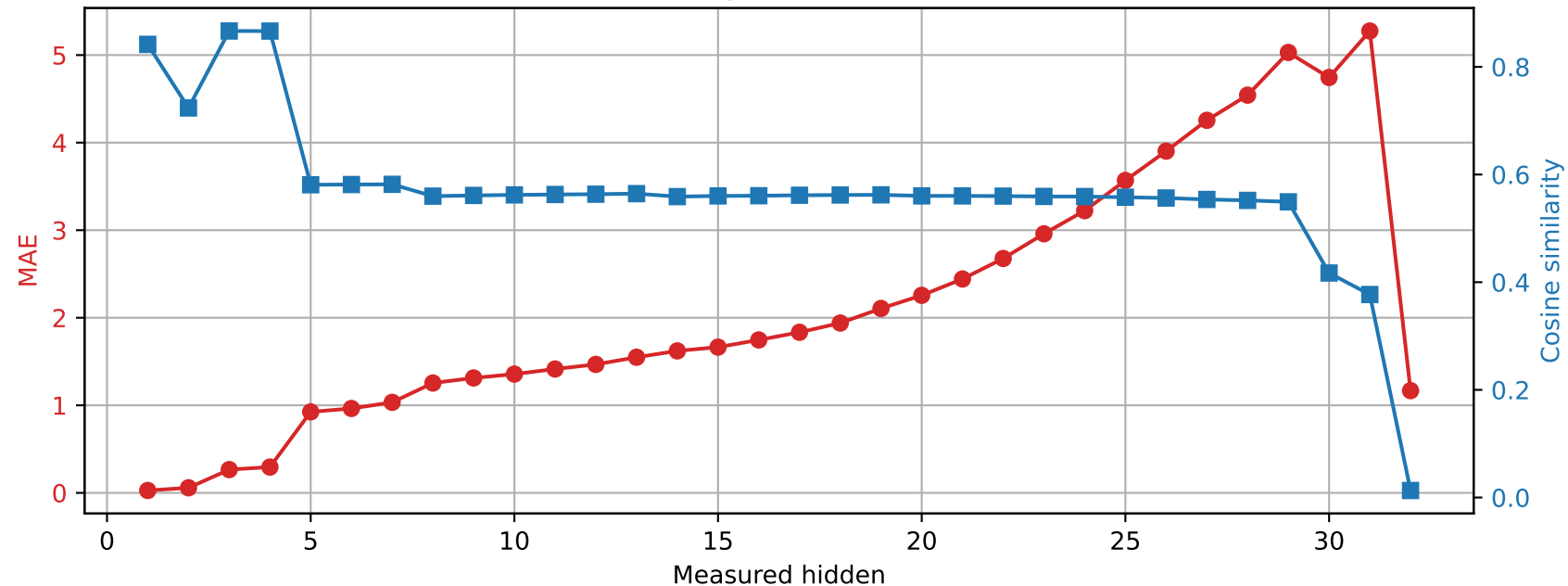
Phi-3-mini-4k-instruct | Prompt 1 Spared layer 12 | Unquantized vs hybrid
