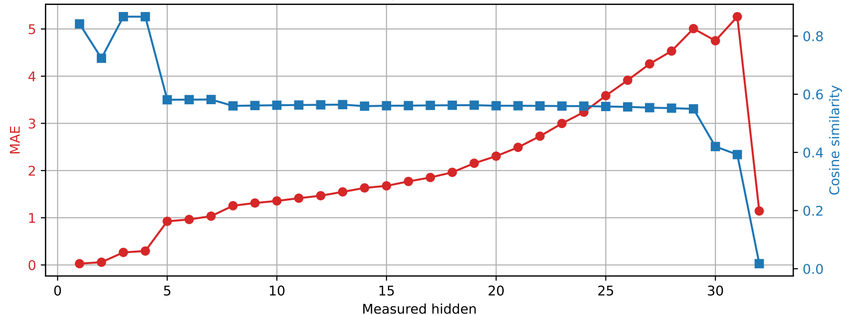
Phi-3-mini-4k-instruct | Prompt 1 Spared layer 13 | Unquantized vs hybrid
