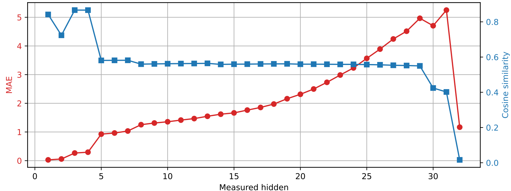
Phi-3-mini-4k-instruct | Prompt 1 Spared layer 23 | Unquantized vs hybrid
