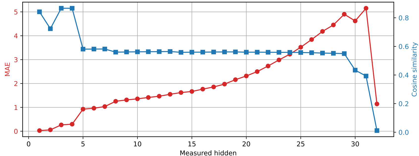
Phi-3-mini-4k-instruct | Prompt 1 Spared layer 24 | Unquantized vs hybrid
