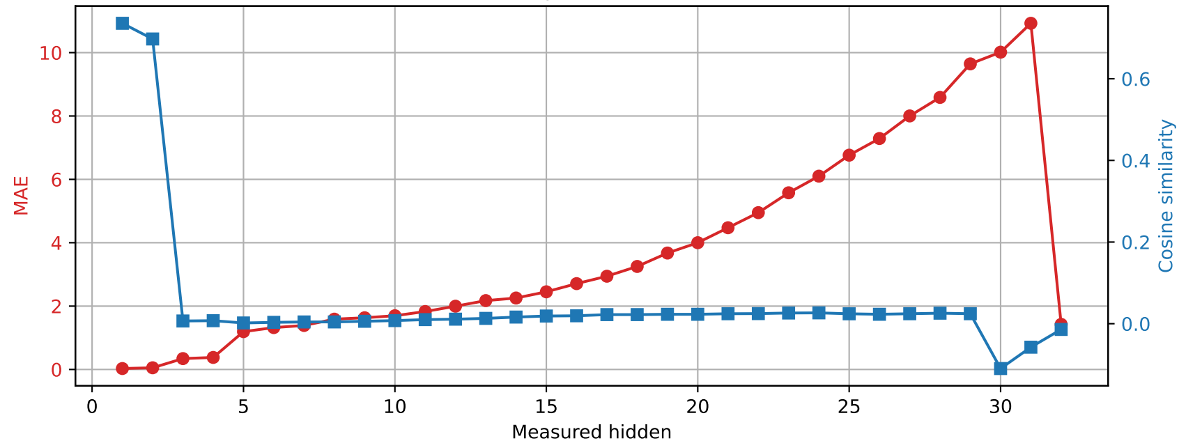
Phi-3-mini-4k-instruct | Prompt 2 Spared layer 5 | Unquantized vs hybrid
