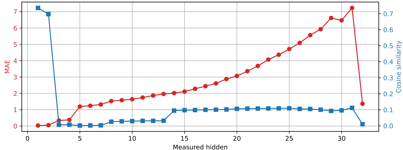
Phi-3-mini-4k-instruct | Prompt 2 Spared layer 24 | Unquantized vs hybrid
