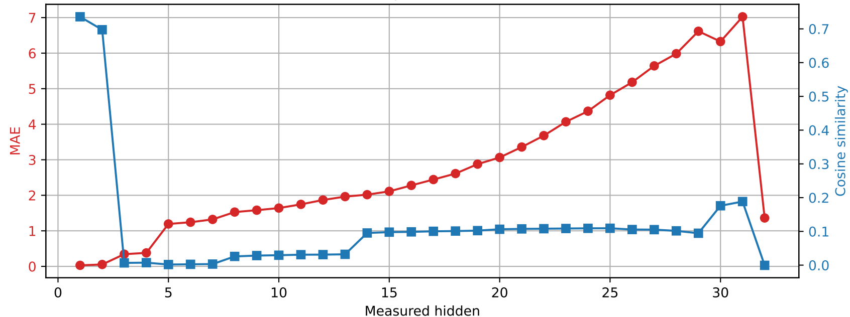
Phi-3-mini-4k-instruct | Prompt 2 Spared layer 27 | Unquantized vs hybrid
