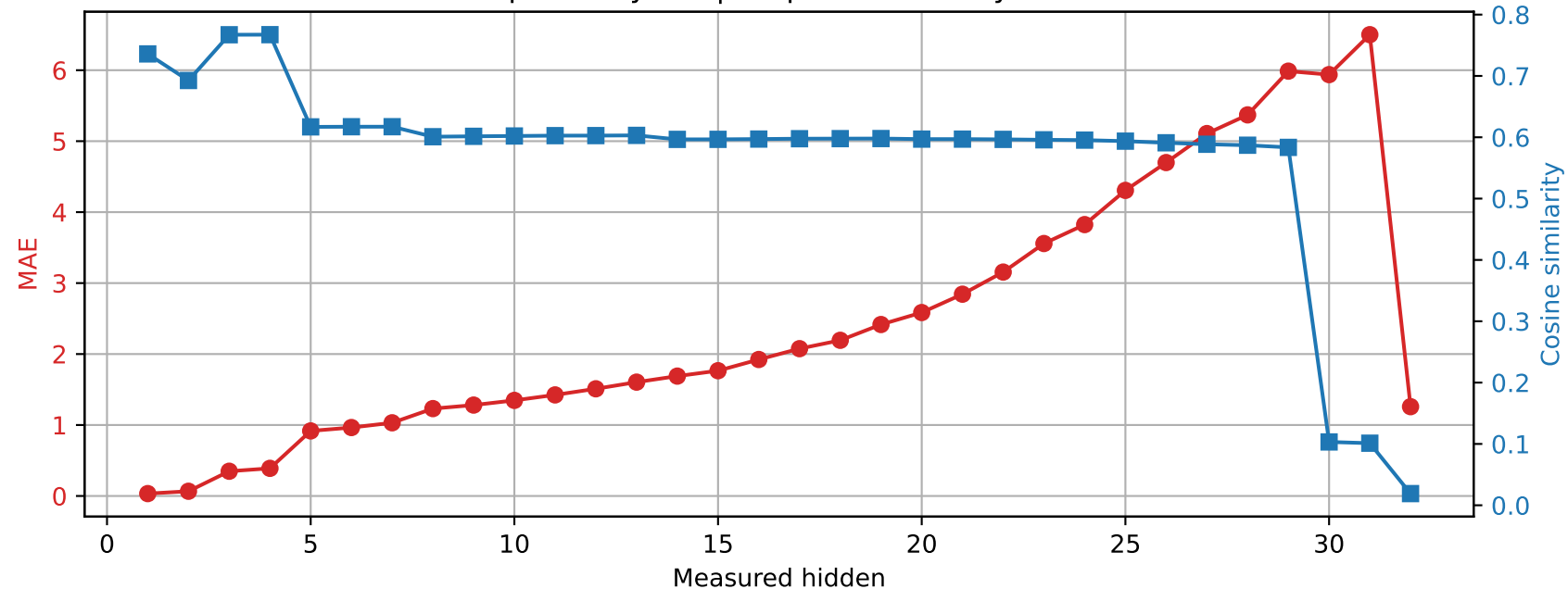
Phi-3-mini-4k-instruct | Prompt 3 Spared layer 4 | Unquantized vs hybrid
