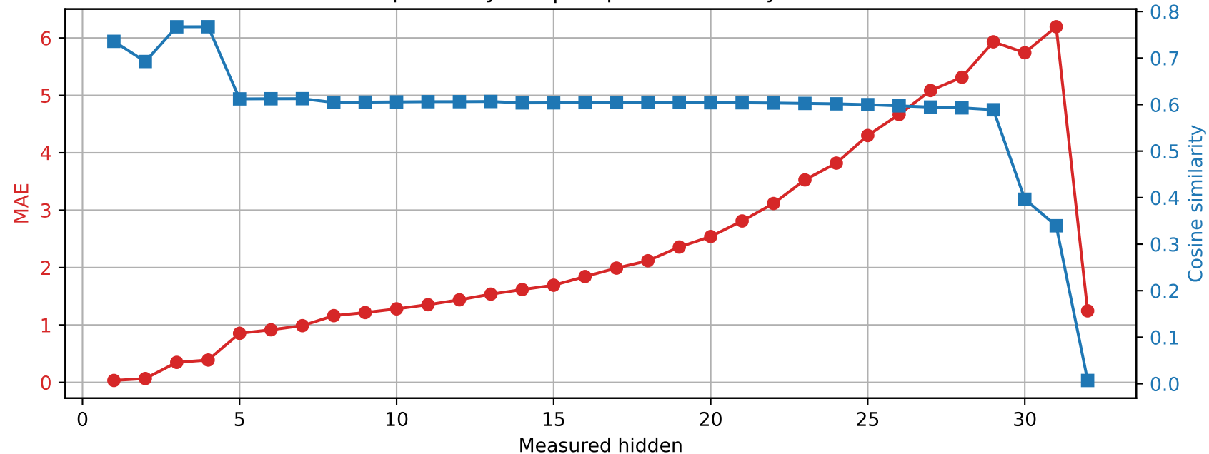
Phi-3-mini-4k-instruct | Prompt 3 Spared layer 5 | Unquantized vs hybrid
