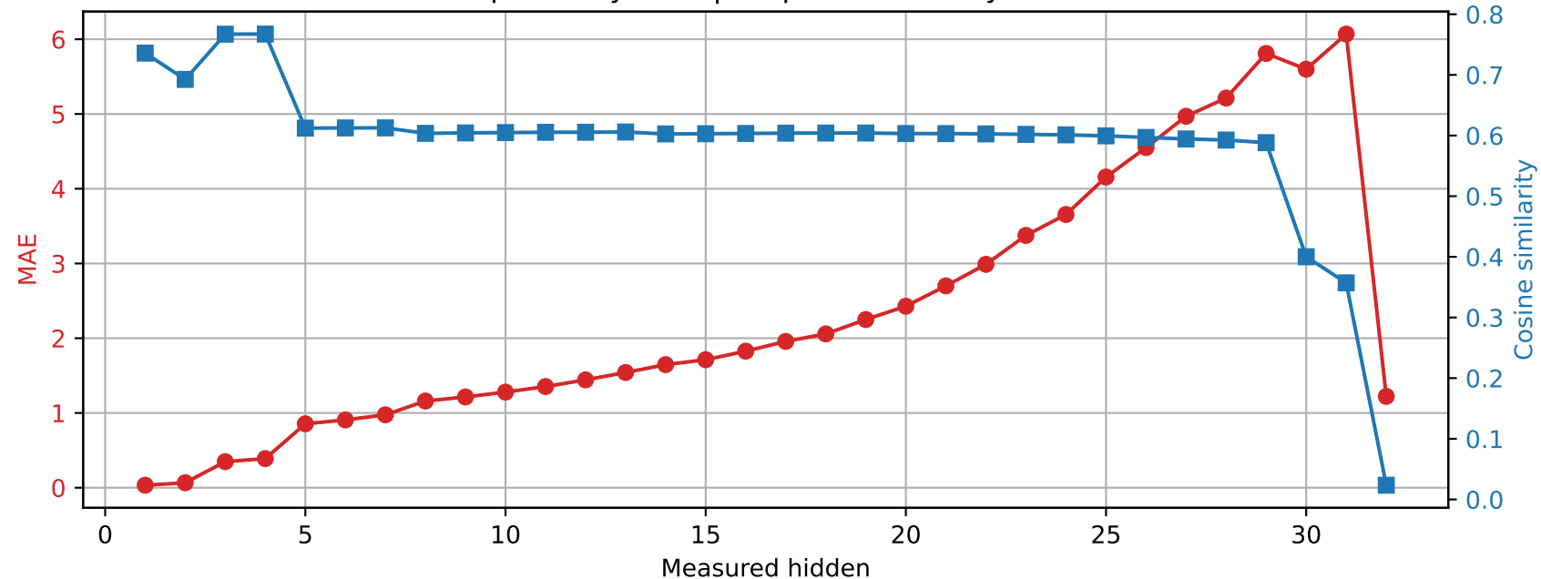
Phi-3-mini-4k-instruct | Prompt 3 Spared layer 13 | Unquantized vs hybrid
