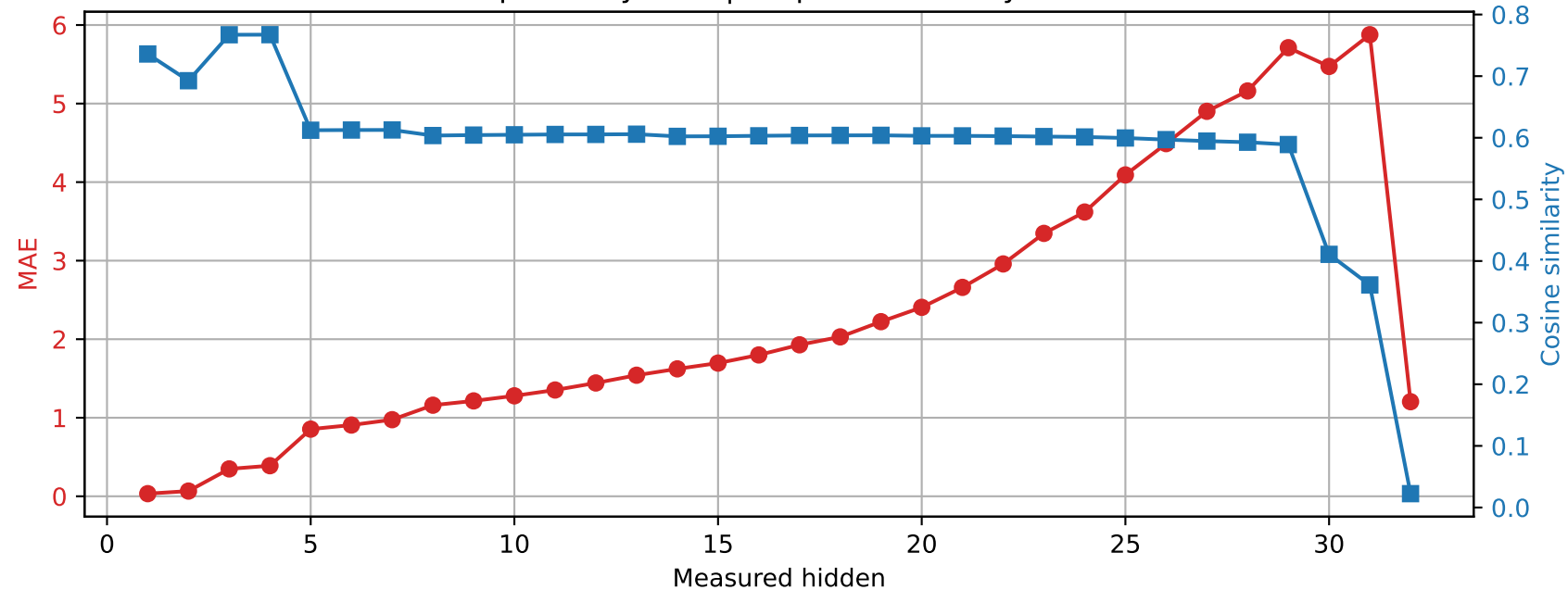
Phi-3-mini-4k-instruct | Prompt 3 Spared layer 15 | Unquantized vs hybrid
