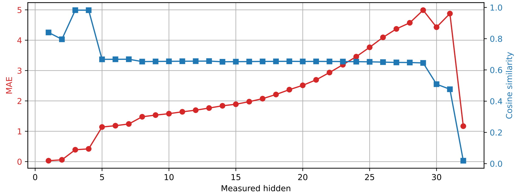
Phi-3-mini-4k-instruct | Prompt 4 Spared layer 17 | Unquantized vs hybrid
