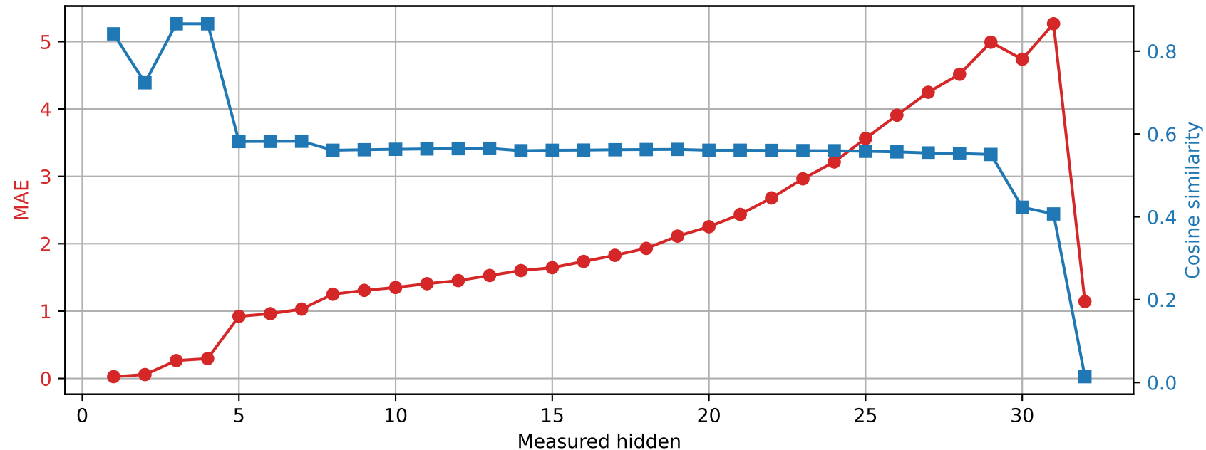
Phi-3-mini-4k-instruct | Prompt 1 Unquantized vs quantized int4
