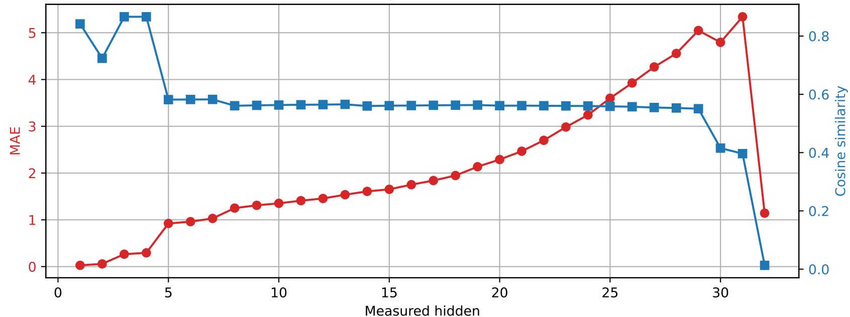
Phi-3-mini-4k-instruct | Prompt 1 Spared layer 8 | Unquantized vs hybrid
