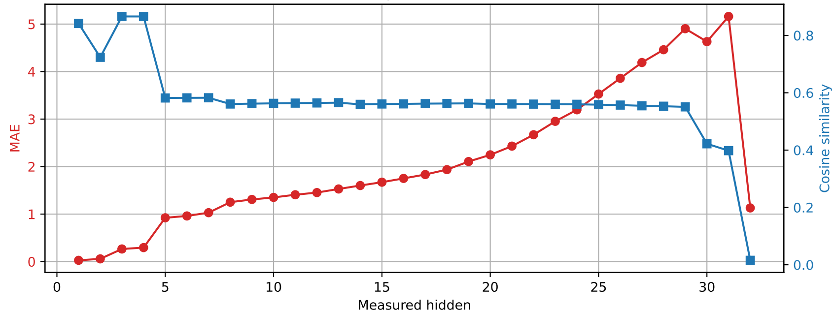
Phi-3-mini-4k-instruct | Prompt 1 Spared layer 14 | Unquantized vs hybrid
