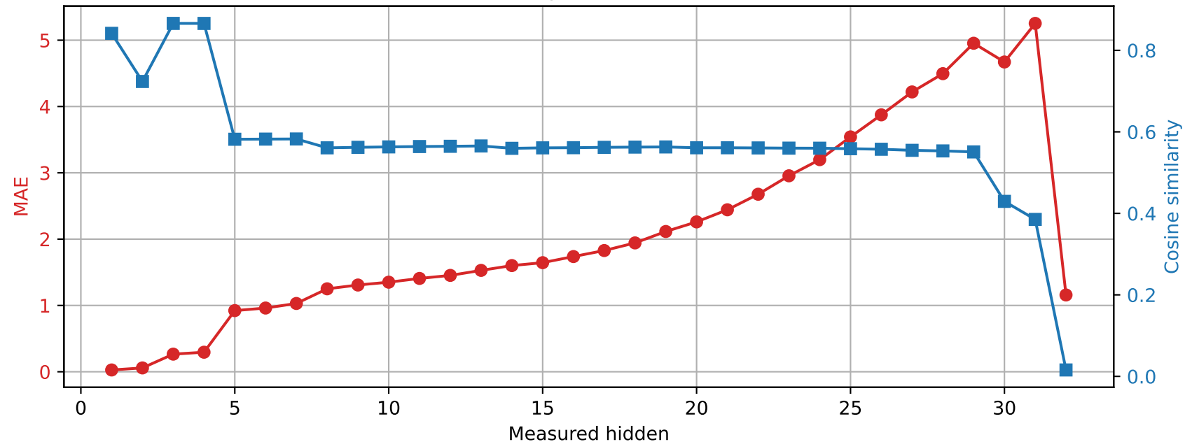
Phi-3-mini-4k-instruct | Prompt 1 Spared layer 17 | Unquantized vs hybrid
