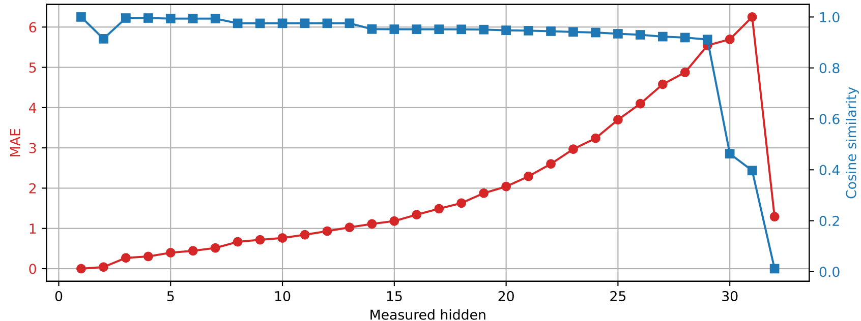
Phi-3-mini-4k-instruct | Prompt 2 Spared layer 0 | Unquantized vs hybrid
