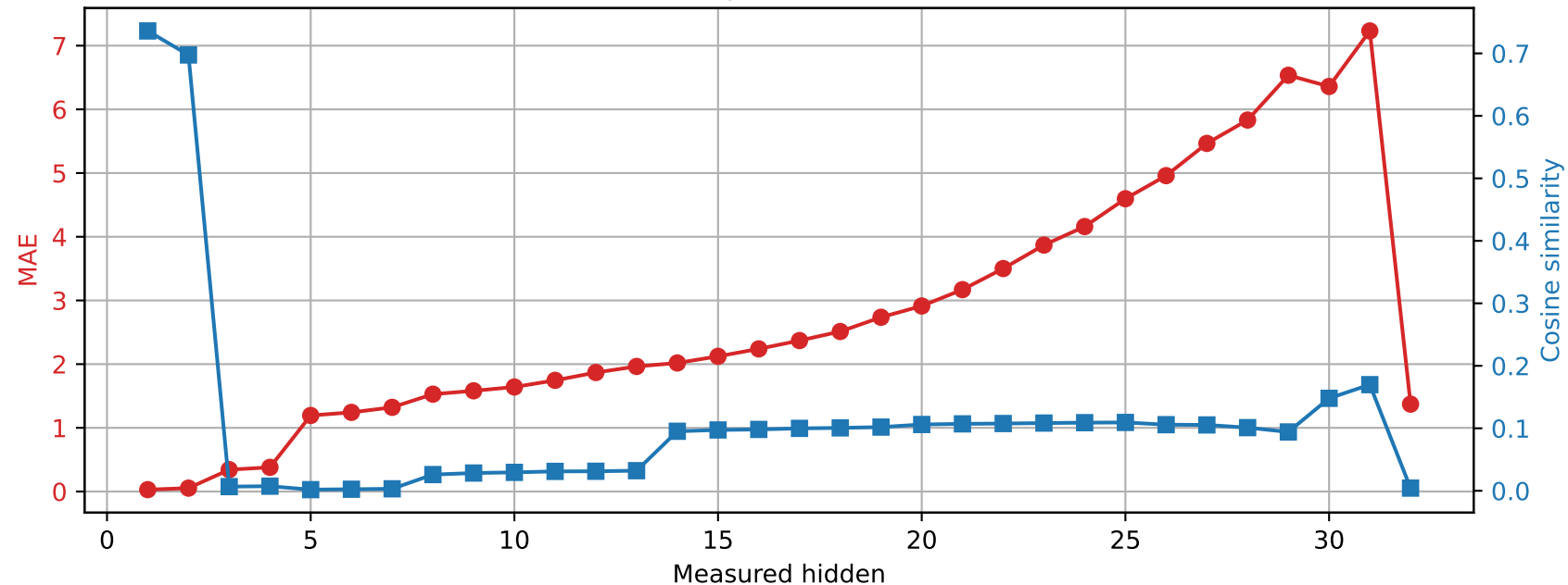
Phi-3-mini-4k-instruct | Prompt 2 Spared layer 14 | Unquantized vs hybrid
