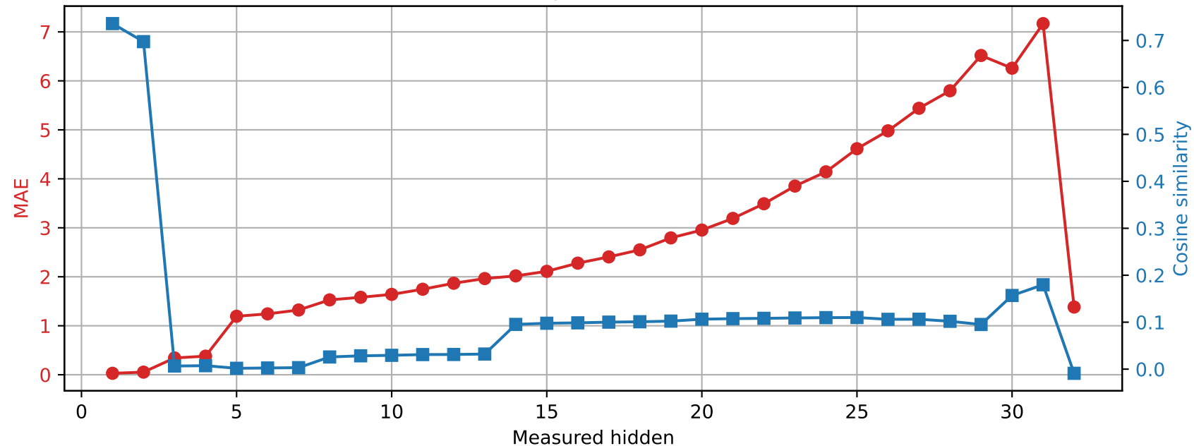
Phi-3-mini-4k-instruct | Prompt 2 Spared layer 16 | Unquantized vs hybrid
