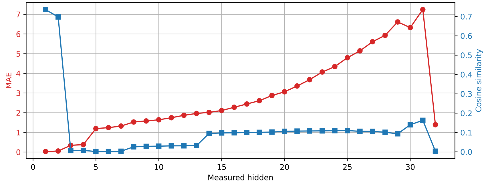
Phi-3-mini-4k-instruct | Prompt 2 Spared layer 23 | Unquantized vs hybrid
