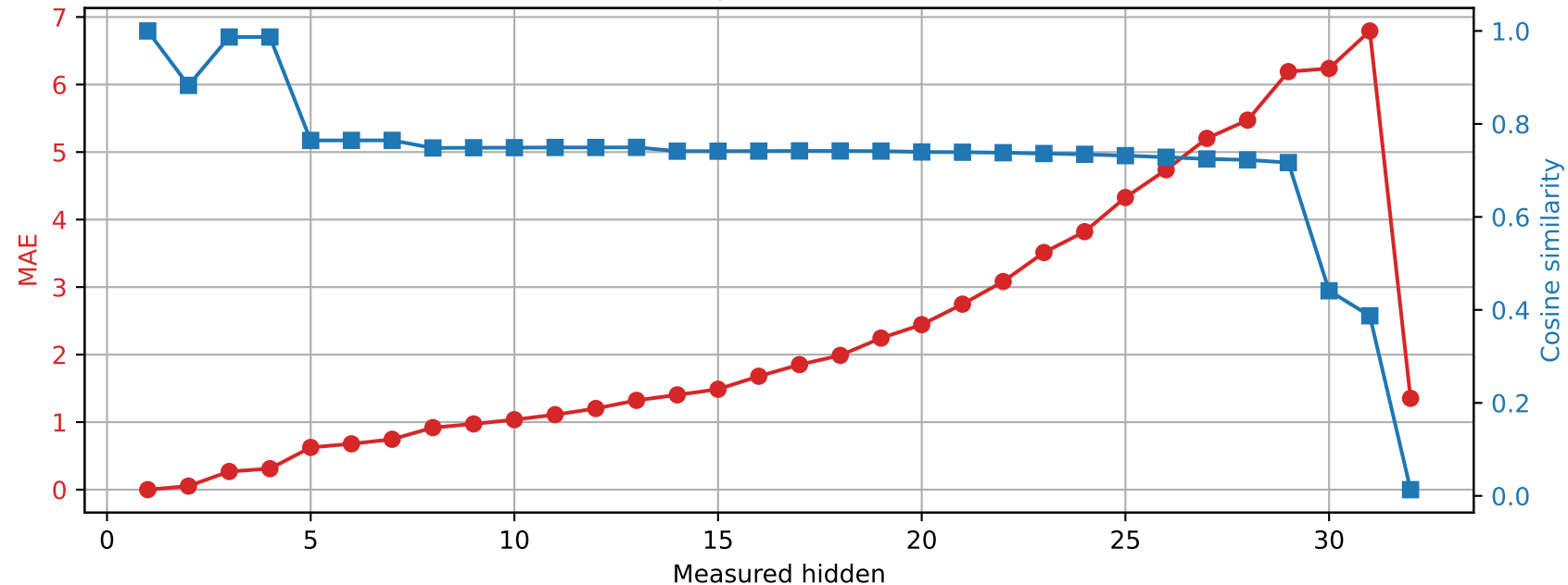
Phi-3-mini-4k-instruct | Prompt 3 Spared layer 0 | Unquantized vs hybrid
