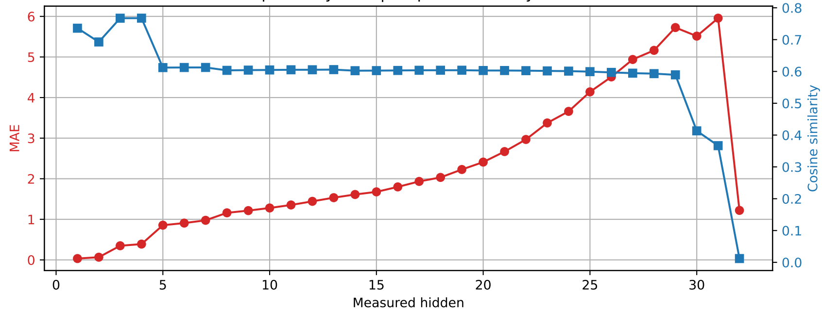
Phi-3-mini-4k-instruct | Prompt 3 Spared layer 12 | Unquantized vs hybrid
