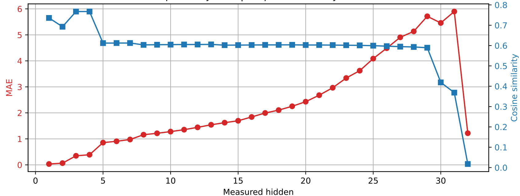
Phi-3-mini-4k-instruct | Prompt 3 Spared layer 18 | Unquantized vs hybrid
