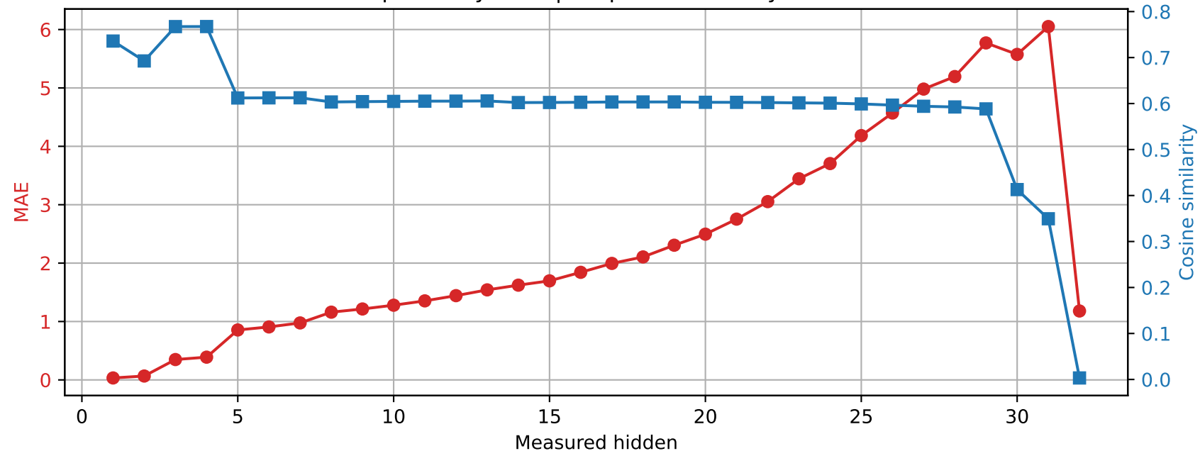
Phi-3-mini-4k-instruct | Prompt 3 Spared layer 19 | Unquantized vs hybrid
