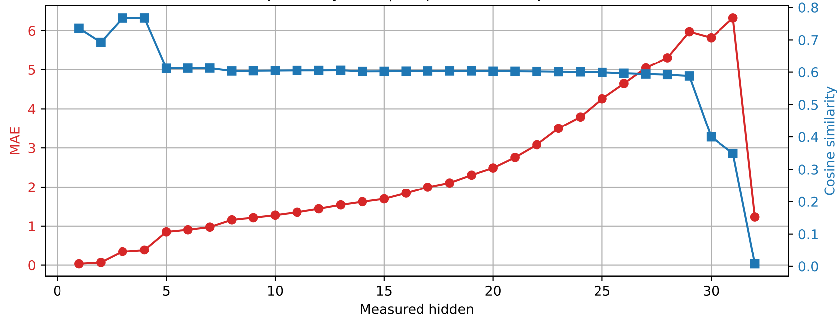
Phi-3-mini-4k-instruct | Prompt 3 Spared layer 23 | Unquantized vs hybrid
