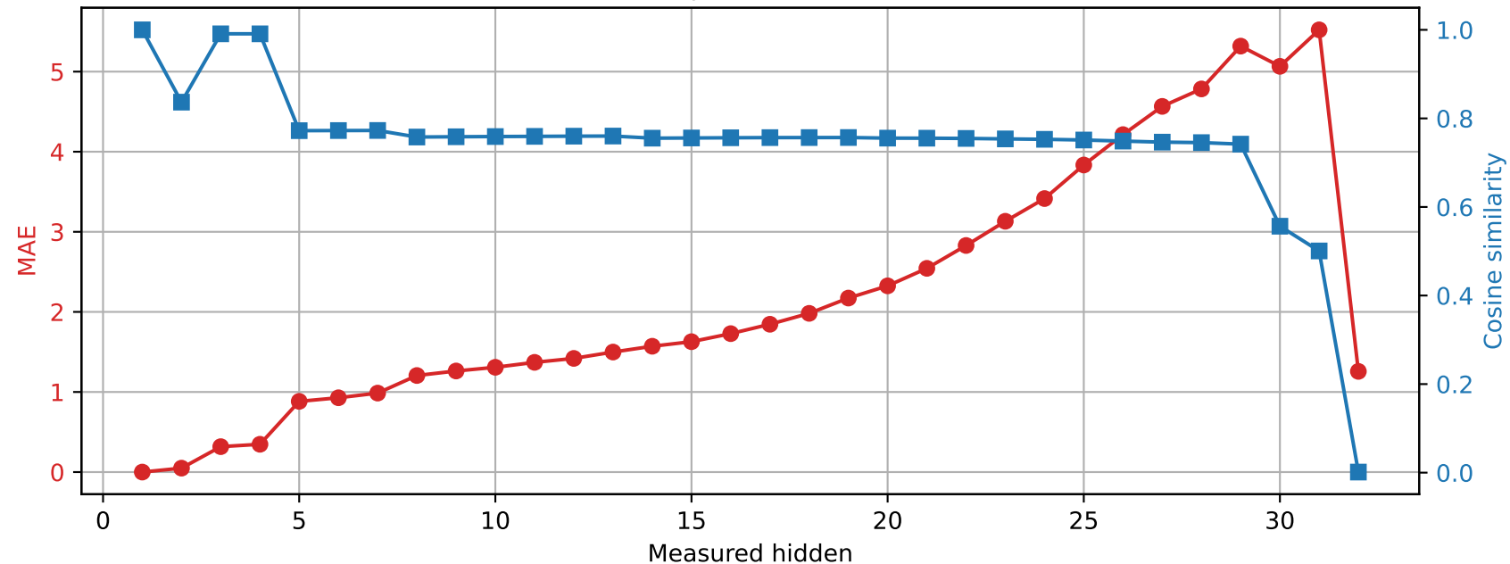
Phi-3-mini-4k-instruct | Prompt 4 Spared layer 0 | Unquantized vs hybrid
