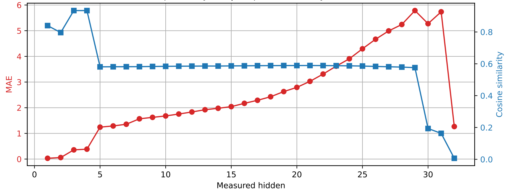
Phi-3-mini-4k-instruct | Prompt 4 Spared layer 2 | Unquantized vs hybrid
