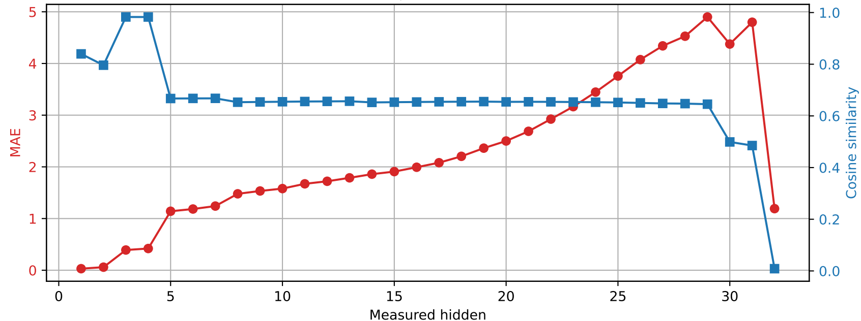
Phi-3-mini-4k-instruct | Prompt 4 Spared layer 10 | Unquantized vs hybrid
