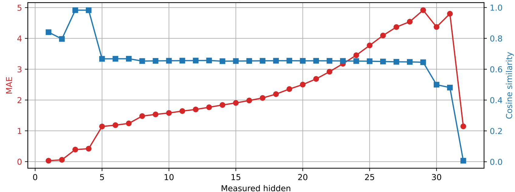
Phi-3-mini-4k-instruct | Prompt 4 Spared layer 14 | Unquantized vs hybrid
