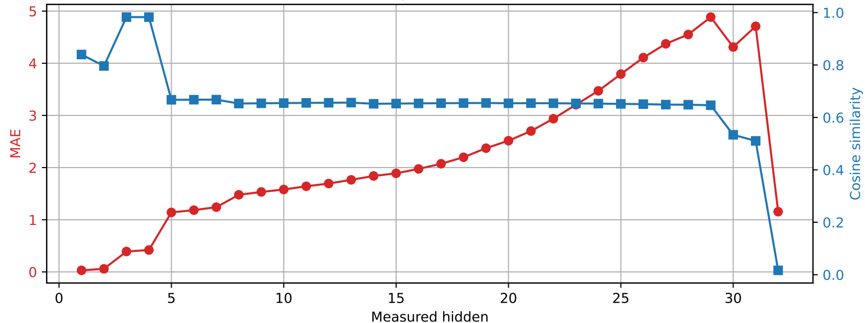
Phi-3-mini-4k-instruct | Prompt 4 Spared layer 25 | Unquantized vs hybrid
