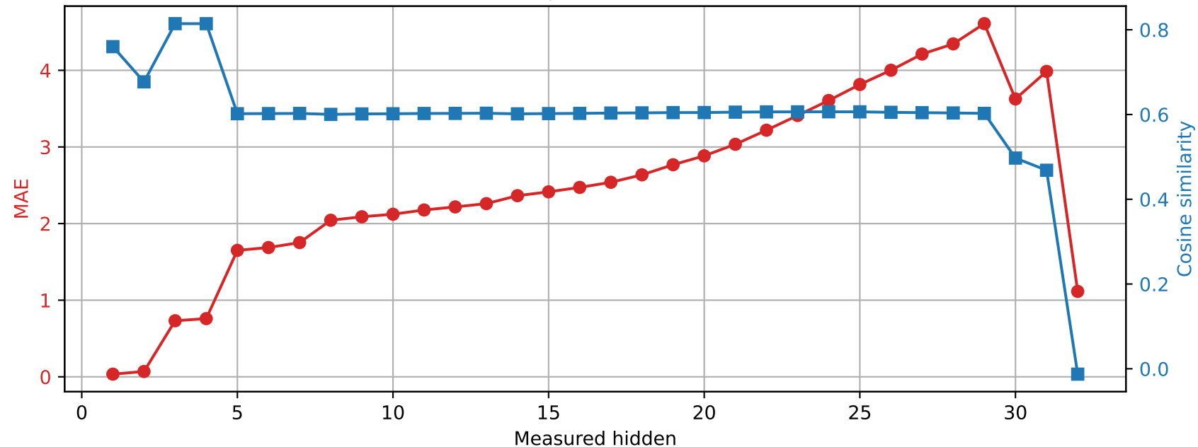
Phi-3-mini-4k-instruct | Prompt 0 Spared layer 9 | Unquantized vs hybrid
