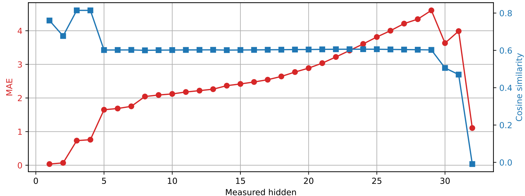
Phi-3-mini-4k-instruct | Prompt 0 Spared layer 18 | Unquantized vs hybrid
