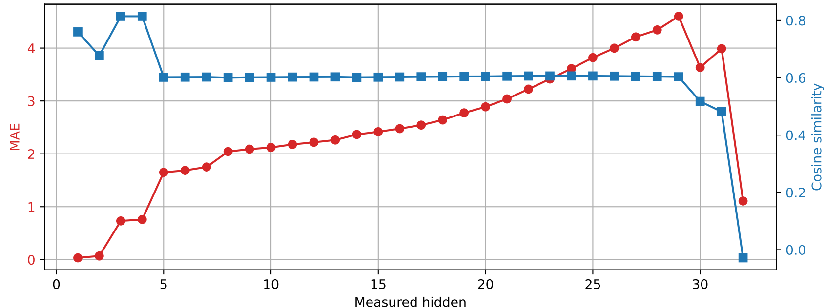
Phi-3-mini-4k-instruct | Prompt 0 Spared layer 25 | Unquantized vs hybrid
