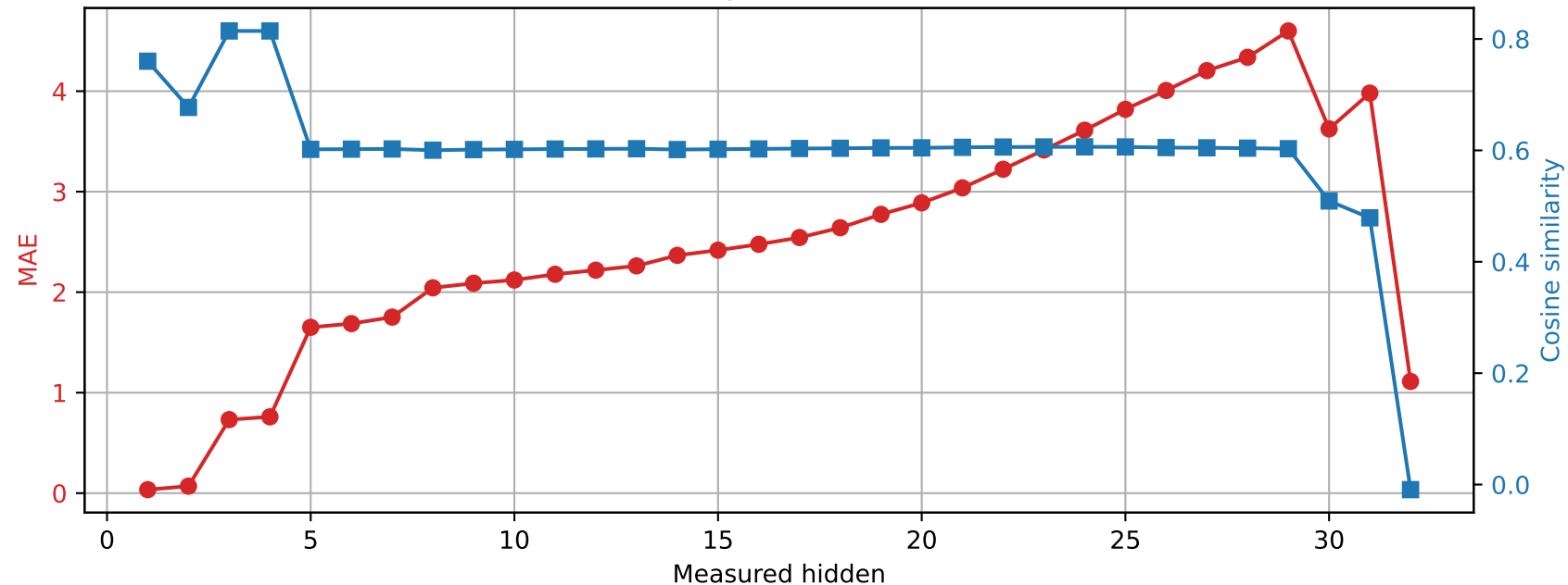
Phi-3-mini-4k-instruct | Prompt 0 Spared layer 26 | Unquantized vs hybrid
