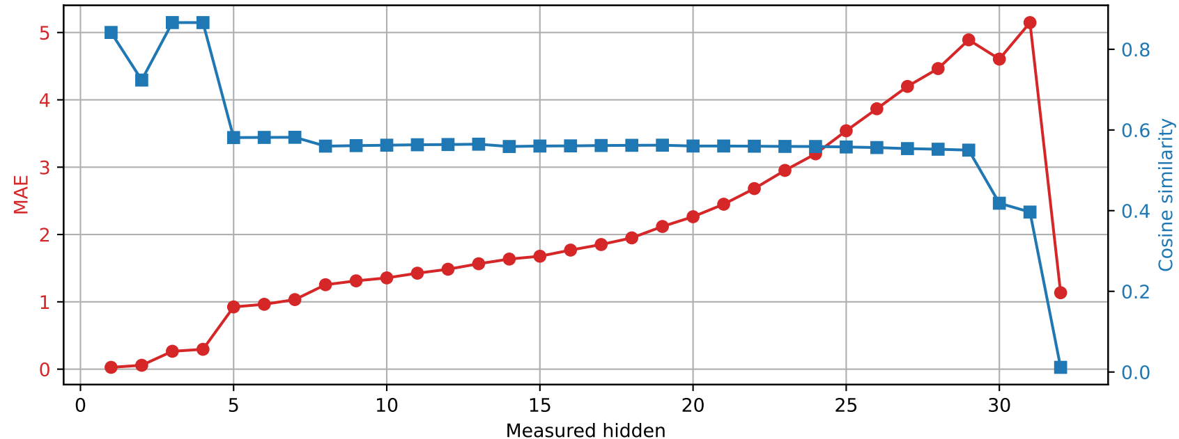
Phi-3-mini-4k-instruct | Prompt 1 Spared layer 10 | Unquantized vs hybrid
