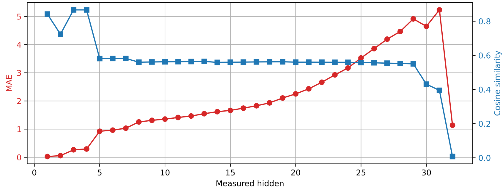
Phi-3-mini-4k-instruct | Prompt 1 Spared layer 15 | Unquantized vs hybrid
