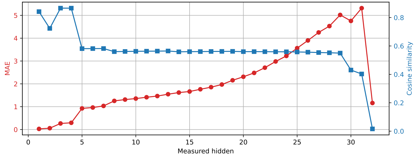
Phi-3-mini-4k-instruct | Prompt 1 Spared layer 20 | Unquantized vs hybrid
