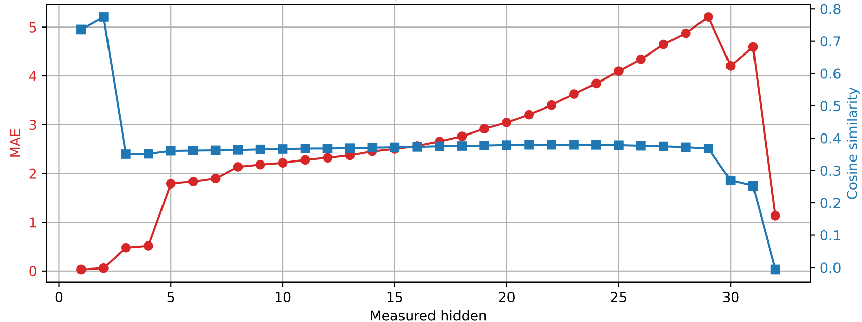
Phi-3-mini-4k-instruct | Prompt 2 Spared layer 1 | Unquantized vs hybrid
