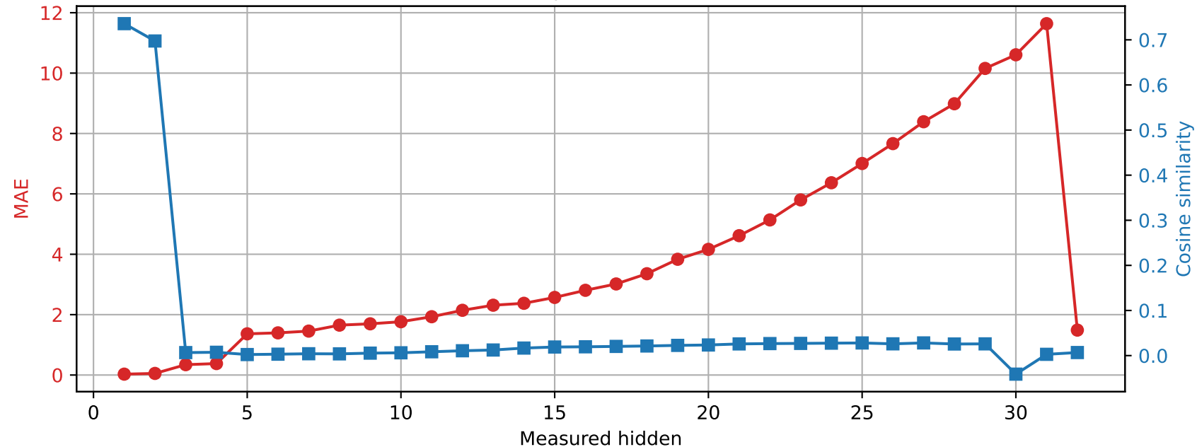
Phi-3-mini-4k-instruct | Prompt 2 Spared layer 4 | Unquantized vs hybrid
