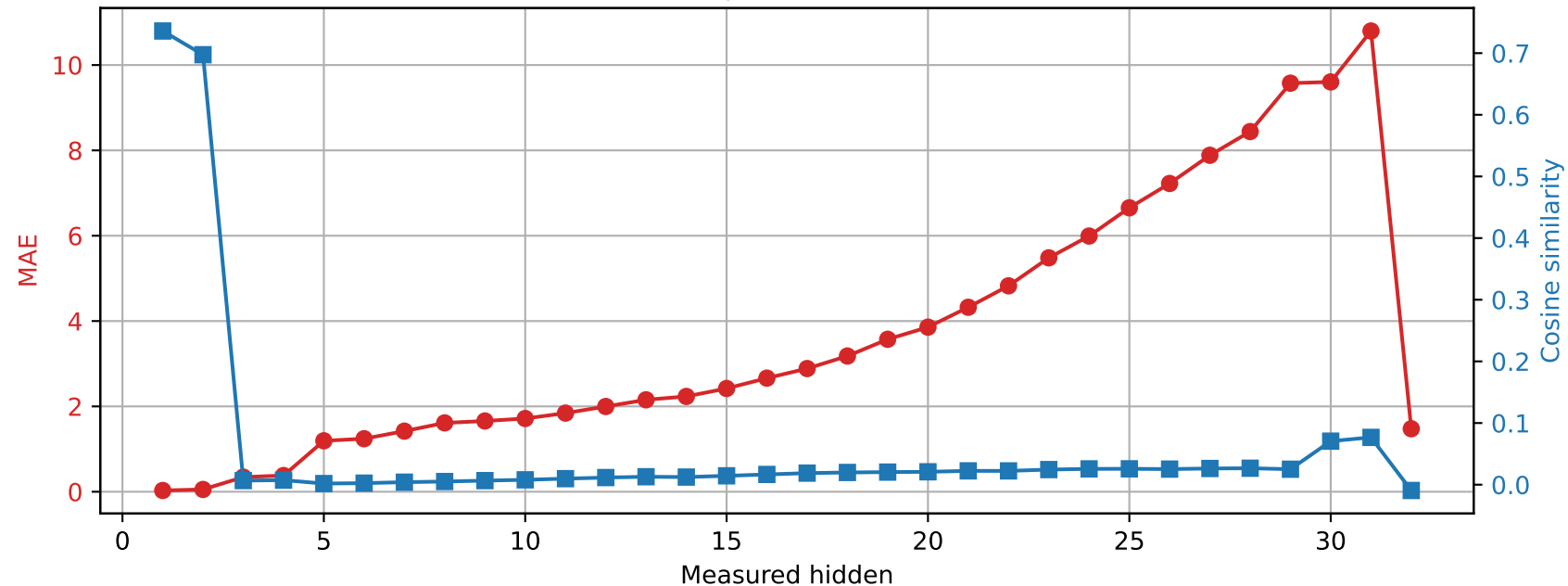
Phi-3-mini-4k-instruct | Prompt 2 Spared layer 6 | Unquantized vs hybrid
